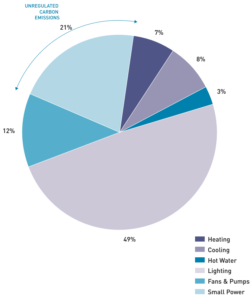
FIGURE 5 BREAKDOWN OF CARBON DIOXIDE EMISSIONS FOR THE BASE CASE SUPERMARKET BUILDING
