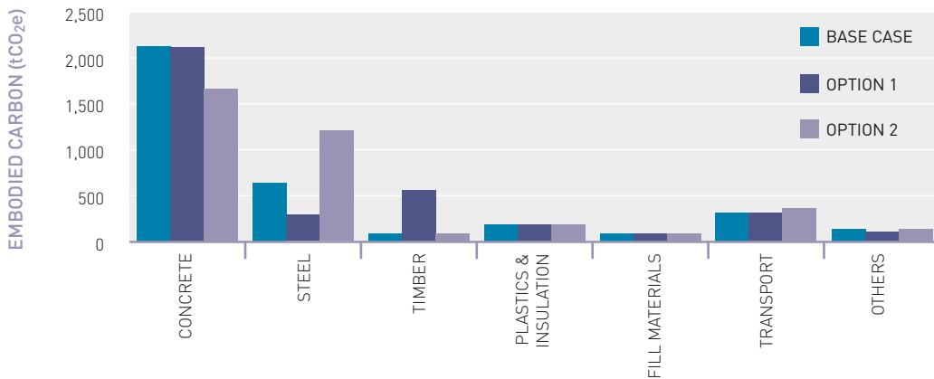
FIGURE 31 BREAKDOWN OF EMBODIED CARBON BY ELEMENT
