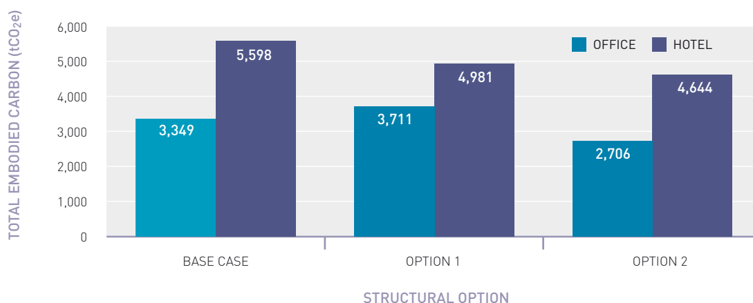
FIGURE 27 TOTAL EMBODIED CARBON EMISSIONS OF THE BASE CASE BUILDING AND STRUCTURAL OPTIONS 1 AND 2
