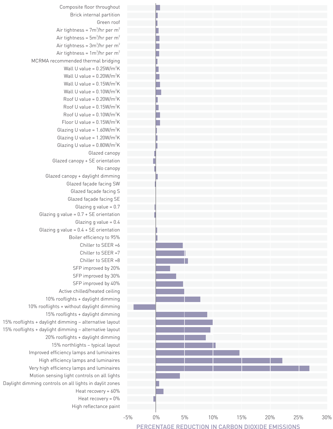
FIGURE 4 REDUCTION IN CARBON DIOXIDE EMISSIONS ACHIEVED BY INTRODUCING ENERGY EFFICIENCY MEASURES (RELATIVE TO THE BASE CASE BUILDING)
