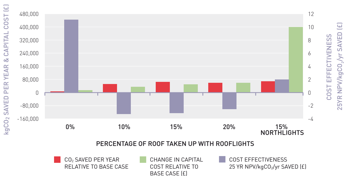
FIGURE 10 MODELLED EFFECTS OF CHANGING ROOFLIGHT AREAS
